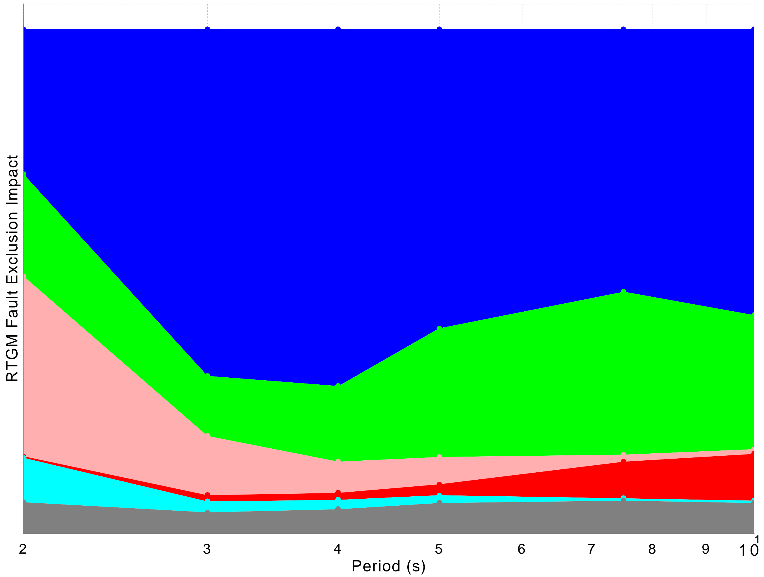
s476 CyberShake MCEr Fault Impact
