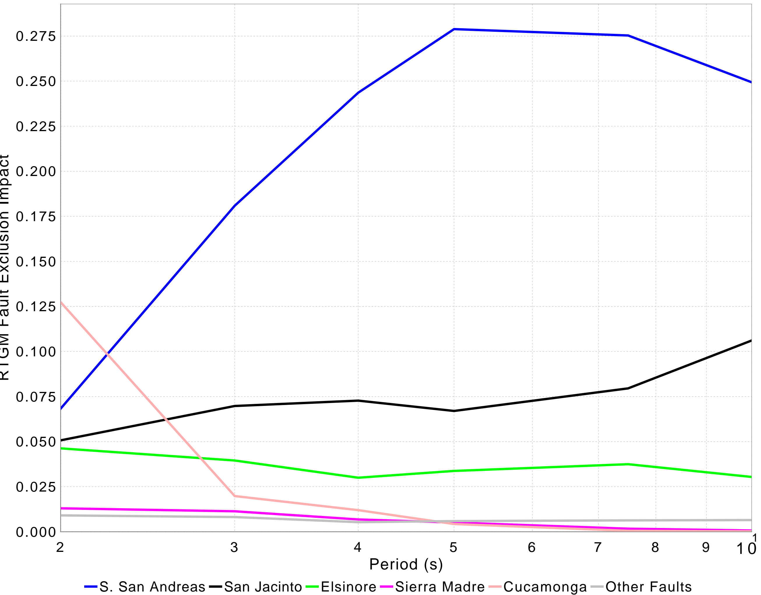
s601 CyberShake MCEr Fault Impact
