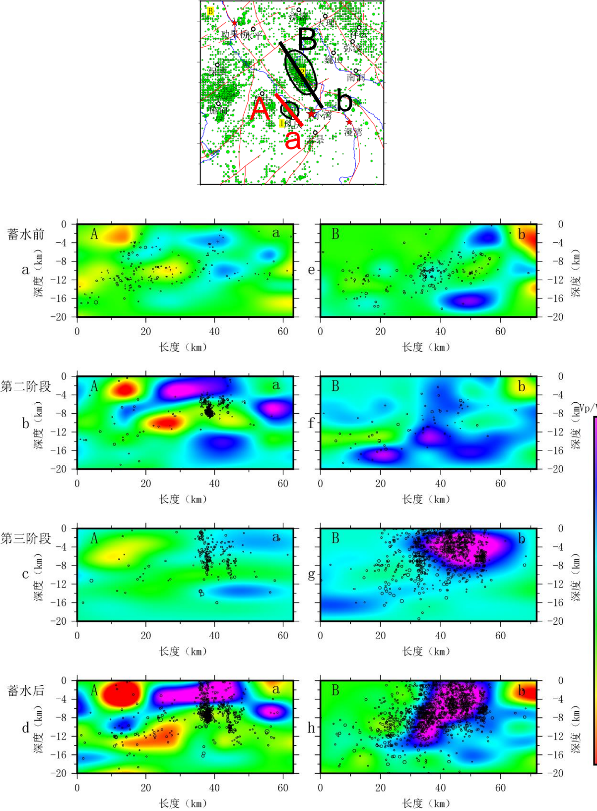
Figure 6. 3-D Vp/Vs tomographic images in vertical depth sections along defined profiles (up) in the Xiaowan reservoir area in different water filling period. a Before the filling, b and c denote the second and third filling phase, respectively. d After the filling. Hypocenters near the profiles within 0.1° are projected as dots. The epicenters are shown as black circles in horizontal planes.
