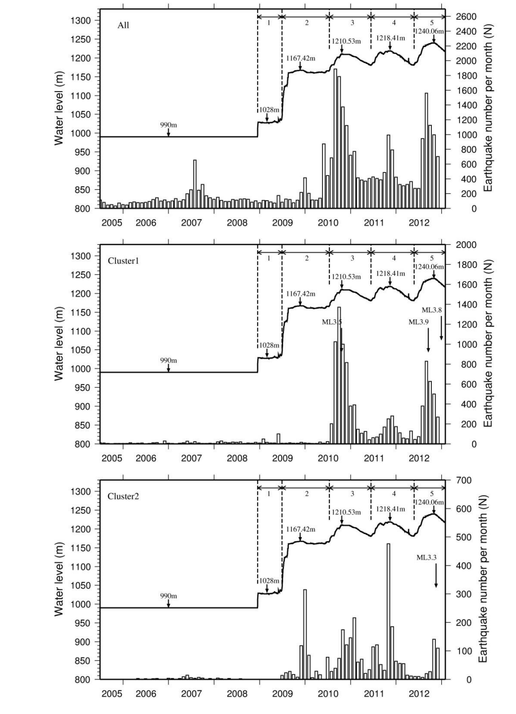
Figure 3 Relation between water level (meters above sea level) and seismicity in the Xiaowan reservoir. There are five water filling periods shown by vertical broken lines in the Xiaowan reservoir. The increase in seismicity in the Xiaowan reservoir was not obvious after the first filling until the third filling began on 15 July 2010. M_L \geq 3.5 in cluster 1 and M_L \geq 3.0 in cluster 2 are shown by vertical arrows.
