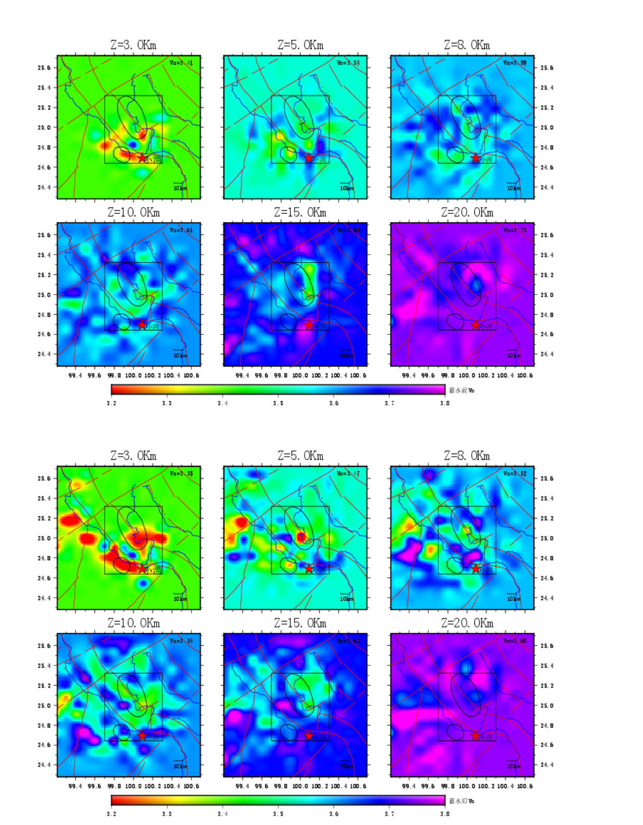
Figure 5. 3-D shear wave velocity images before (up) and after (down) the impoundment, measured by the local earthquake tomography method SIMUL2000. Low-Vs anomalies after the impoundment can be found beneath and around the Lancang River and the Heihui River in the reservoir area, where the two clusters are located.
