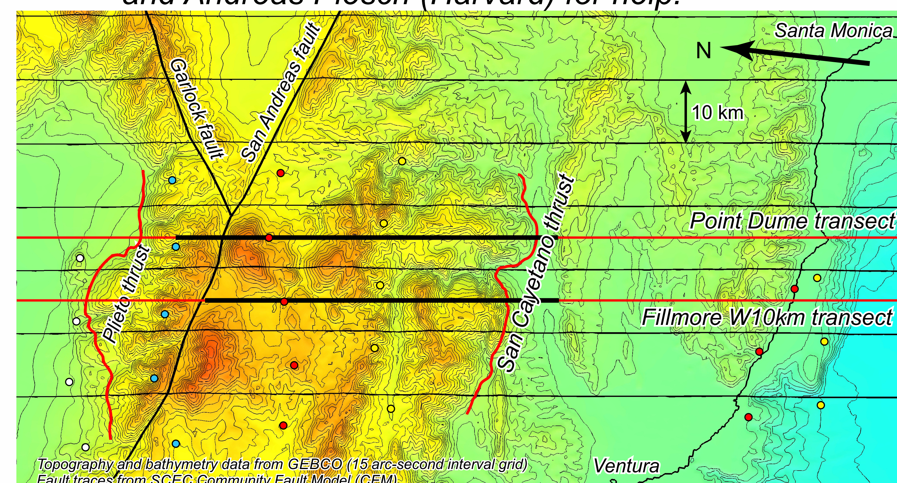
Regional velocity inversion
