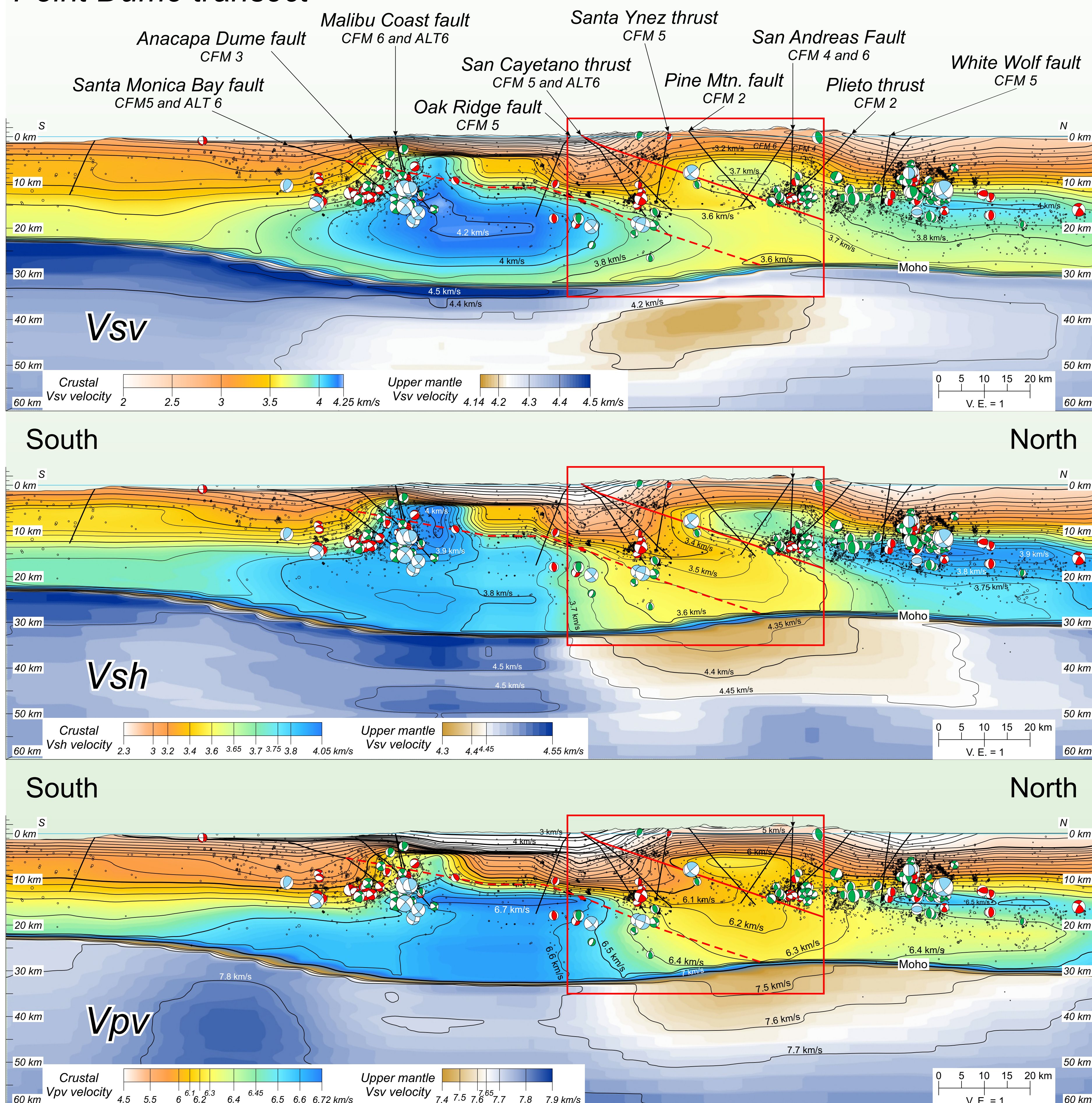
Point Dume transect
