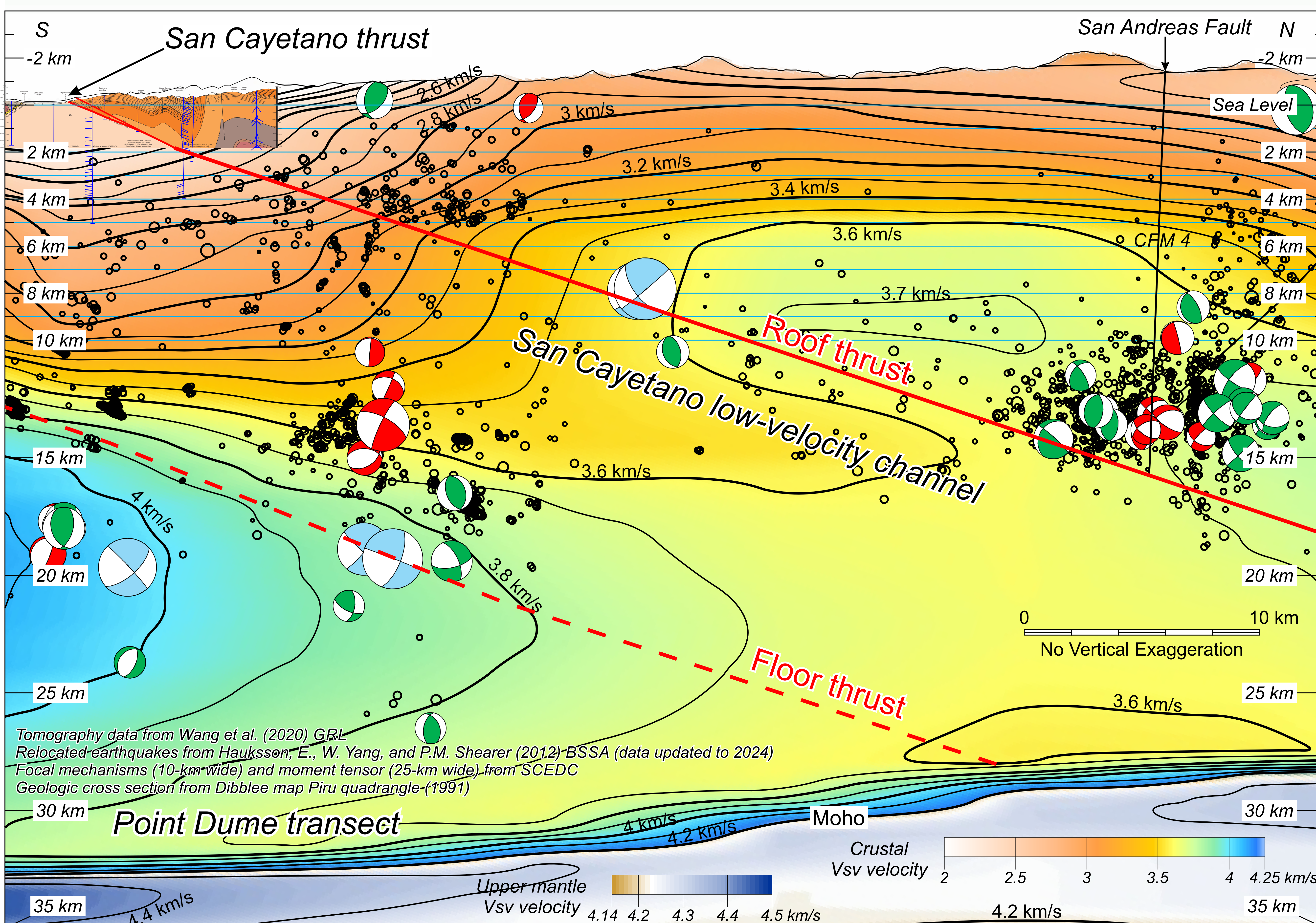
Point Dume transect
