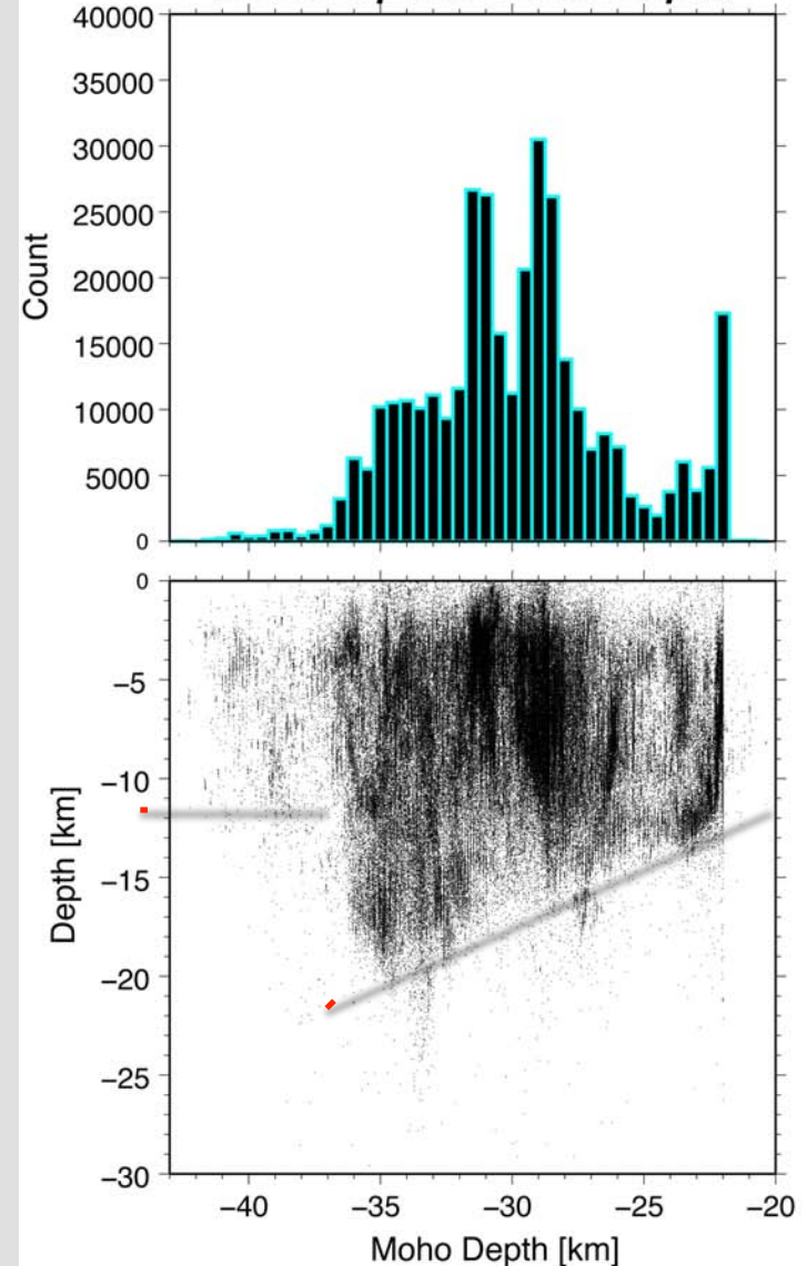
Focal Depths & Moho Depth
