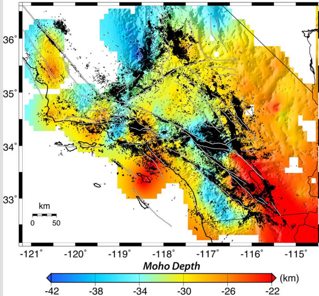
Moho Depth From Receiver Functions, modified from (Yan and Clayton, 2007) Relocated Seismicity 1981 - 2005
